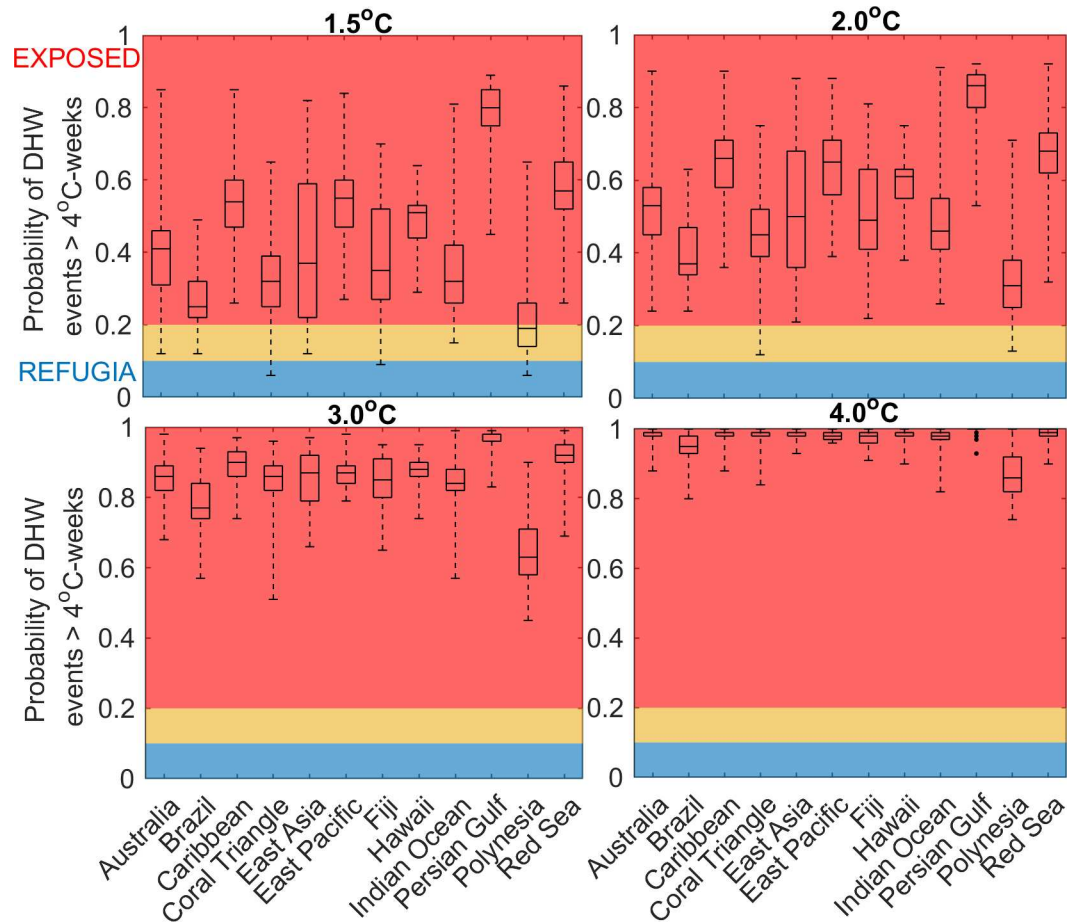
Fig 3. Probability of DHW events > 4°C-weeks across 12 coral reef regions under 1.5, 2.0, 3.0 and 4.0°C of global warming relative to pre-industrial levels. Thresholds for determining thermal refugia (probability of DHW events > 4°C-weeks less than 0.1 yr -1 ) and exposed reefs (probability of DHW events > 4°C-weeks greater than 0.2 yr -1 ) are represented by the blue and red shaded areas, respectively.
