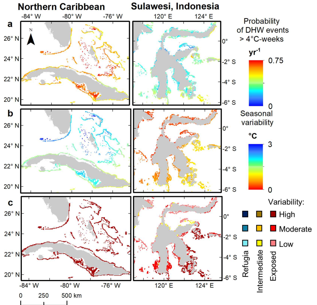
Fig 5. Probability of DHW events > 4^{\circ}\text{C-weeks} (a), seasonal SST variability (b) and exposure category (c) in the Northern Caribbean and Sulawesi, Indonesia at 1.5^{\circ}\text{C} of global warming. Exposure categories are thermal refugia (probability of DHW events > 4^{\circ}\text{C-weeks} less than 0.1\text{ yr}^{-1} ), intermediate (probability of DHW events > 4^{\circ}\text{C-weeks} from 0.1\text{--}0.2\text{ yr}^{-1} ) and exposed (probability of DHW events > 4^{\circ}\text{C-weeks} greater than 0.2\text{ yr}^{-1} ). Exposure categories are split by the level of SST variability (high = seasonal OR inter-annual variability > 0.7^{\circ}\text{C} , low = seasonal AND inter-annual variability < 0.3^{\circ}\text{C} , moderate = all others). The base map is made with Natural Earth.
