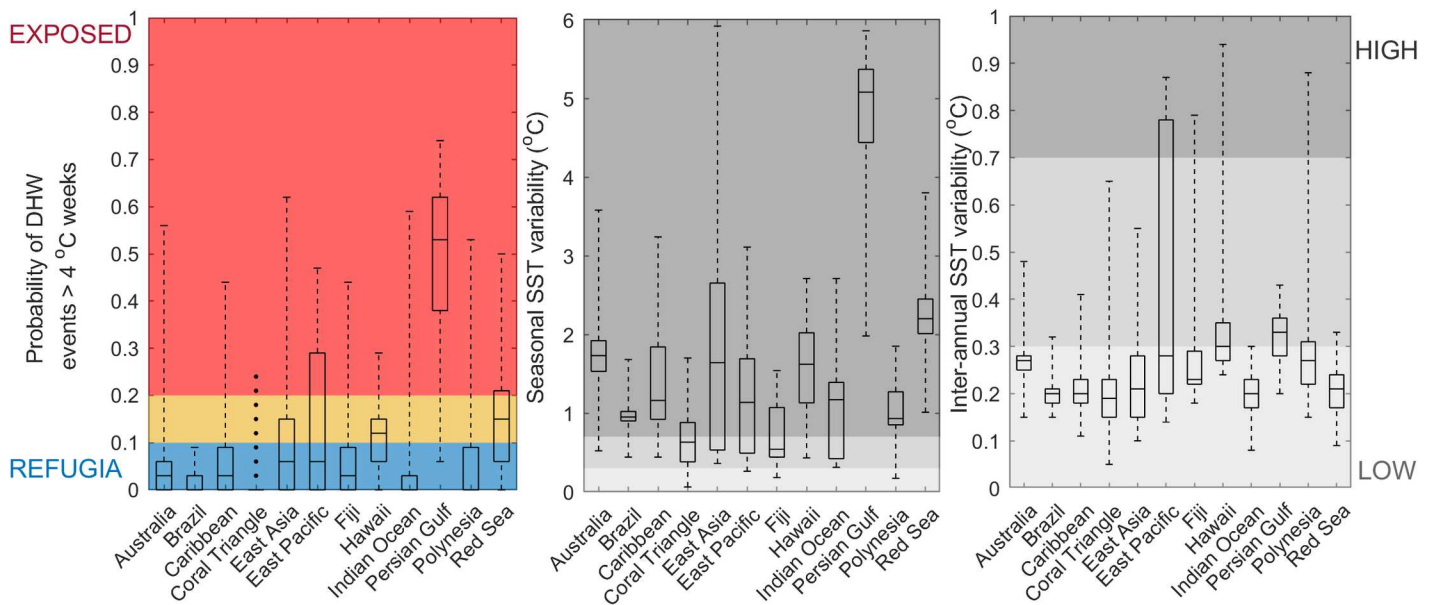
Fig 1. Probability of DHW events > 4°C-weeks, seasonal SST variability and inter-annual SST variability in 12 coral reef regions during the period 1986–2019. Outliers (>100 * interquartile range) are shown by the black dots. Thresholds for determining thermal refugia (probability of DHW events > 4°C-weeks less than 0.1 yr -1 ) and exposed reefs (probability of DHW events > 4°C-weeks greater than 0.2 yr -1 ) are represented by the blue and red shaded areas, respectively. Thresholds for determining high SST variability (> 0.7°C) and low SST variability (< 0.3°C) are represented by the dark and light grey shaded areas, respectively.
