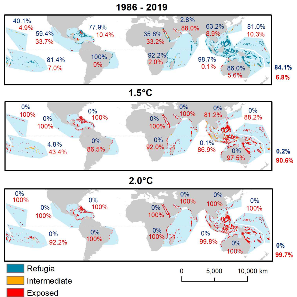
Fig 2. Global distribution of exposure category in the 1986–2019 climate and at 1.5 and 2.0°C of future global warming. Exposure categories are thermal refugia (probability of DHW events > 4°C-weeks less than 0.1 yr -1 ), intermediate (probability of DHW events > 4°C-weeks from 0.1–0.2 yr -1 ) and exposed (probability of DHW events > 4°C-weeks greater than 0.2 yr -1 ). Percentages indicate the regional (on map) and global (right of map) proportion of thermal refugia (blue) and exposed reefs (red). The 12 coral reef regions are outlined in light blue. The base map is made with Natural Earth.
