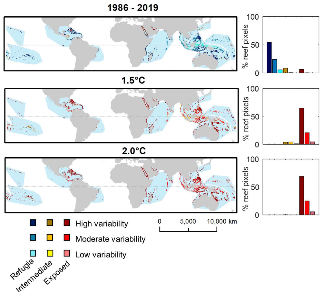
Fig 4. Global distribution of exposure category and SST variability level in the 1986–2019 climate and at 1.5 and 2.0°C of future global warming relative to pre-industrial levels. Exposure categories are thermal refugia (probability of DHW events > 4°C-weeks less than 0.1 yr -1 ), intermediate (probability of DHW events > 4°C-weeks from 0.1–0.2 yr -1 ) and exposed (probability of DHW events > 4°C-weeks greater than 0.2 yr -1 ). Exposure categories are split by the level of SST variability (high = seasonal OR inter-annual variability > 0.7°C, low = seasonal AND inter-annual variability < 0.3°C, moderate = all others). The 12 coral reef regions are outlined in light blue. Bars indicate the percentage of 1 km reef pixels in each exposure category. The base map is made with Natural Earth.
