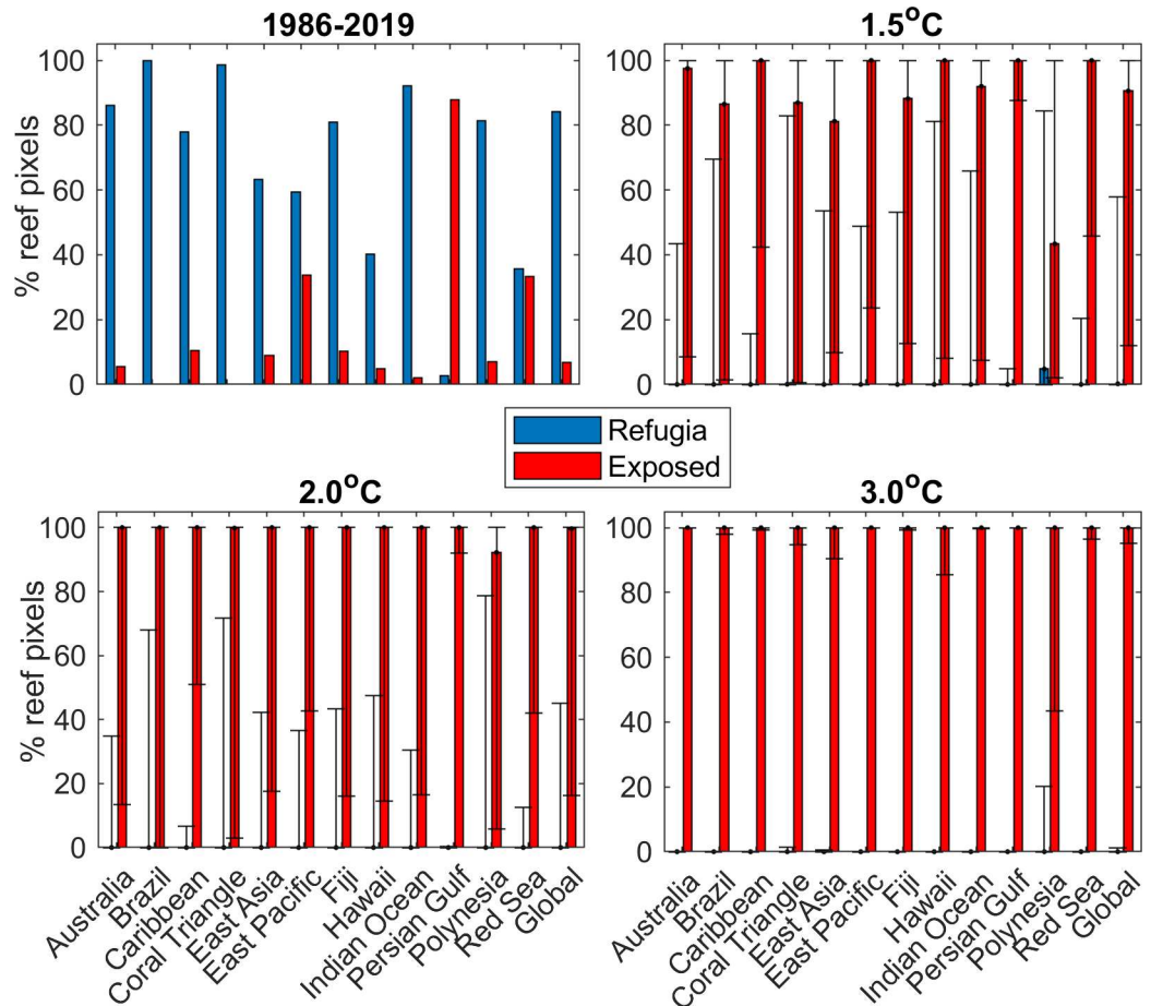
Fig 6. Percentage of thermal refugia and exposed reef pixels in 12 coral reef regions and globally in the 1986–2019 climate and at 1.5, 2.0 and 3.0°C of global warming. As with 3.0°C, there are 0% thermal refugia and 100% exposed reefs at 4.0°C of global warming. Error bars are the percentage of thermal refugia and exposed reefs identified using the maximum and minimum probability of DHW events > 4^\circ\text{C} -weeks simulated by the 57 sets of CMIP6 climate projections (15 models and four SSP emissions scenarios: two climate models, GFDL-CM4 and NESM3, had only two and three SSP runs available, respectively).
